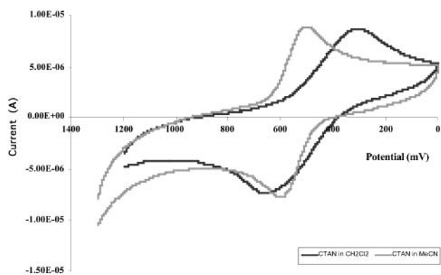
Figure 1. Cyclic voltammograms of CTAN at a glassy carbon electrode in acetonitrile and \text{CH}_2\text{Cl}_2 vs \text{Ag}/\text{AgNO}_3 reference electrode.
